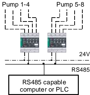
Figure 2.1, Example of a simple configuration with DigiCon-Modbus
